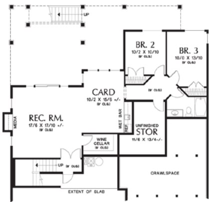
daylight basement
