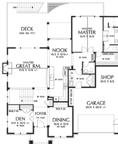
main floor
